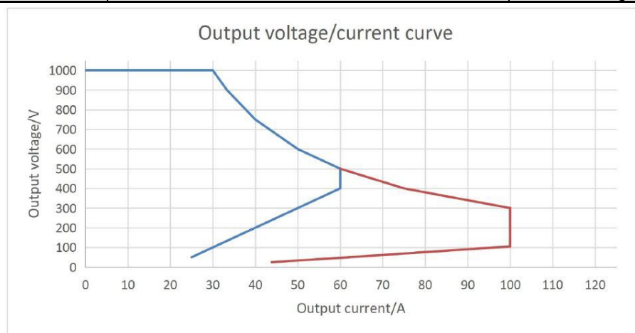
Fig. 2 Output Power Curve
