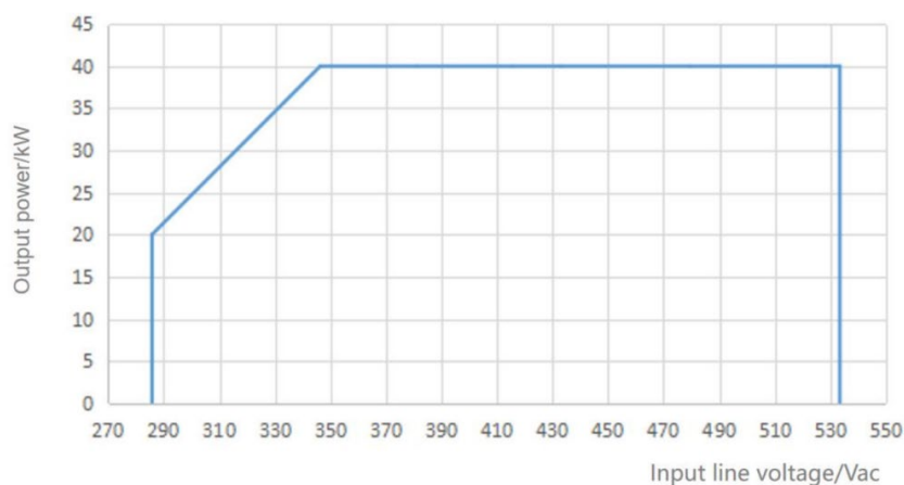
Fig. 1 Input Power Curve
