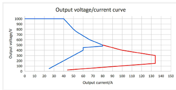
Fig. 2 Output Power Curve
