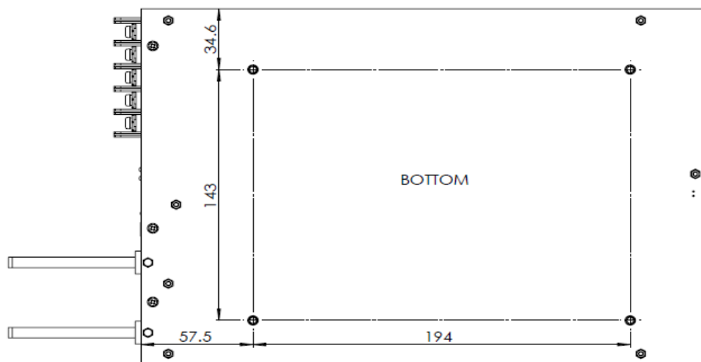
Bottom View
