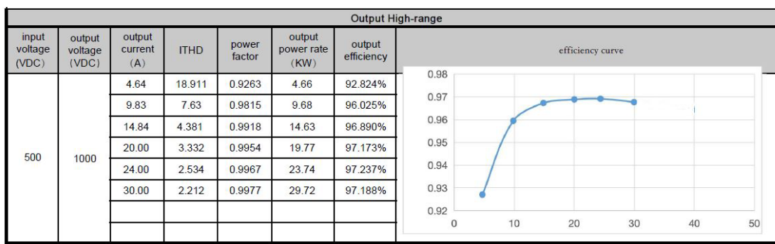
Fig. 2 Efficiency Curve
