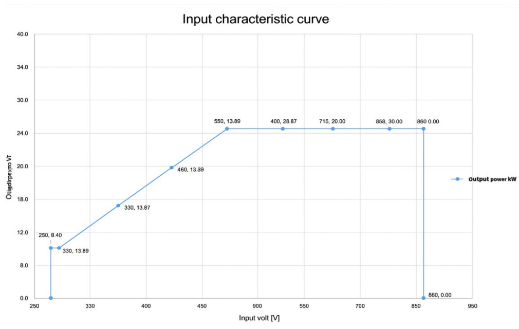
Fig. 1 Input Power Curve
