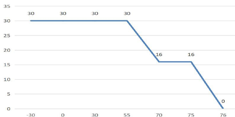
Ambient Temperature Limit Power Curve
