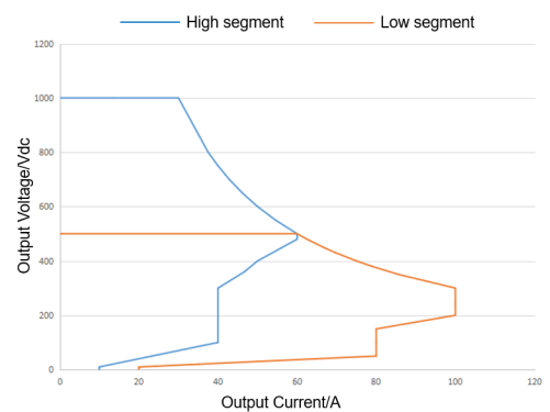
Fig. 3 Output Power Curve
